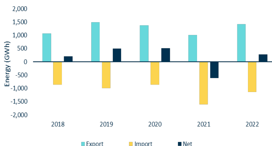
Figure 19: Basslink exports and imports, as at 30 June 2018-2022 (Hydro Tasmania, 2022)
