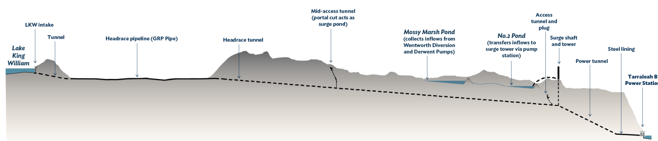
Figure 11: The proposed redeveloped Tarraleah scheme
