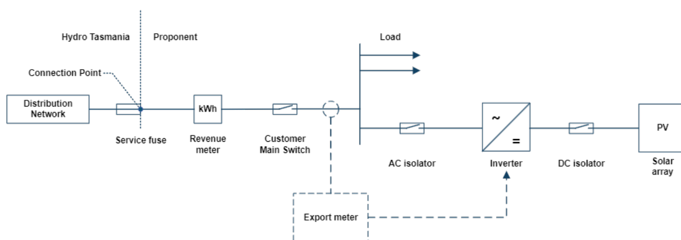
Figure 1: Single line diagram for a solar inverter connection.
